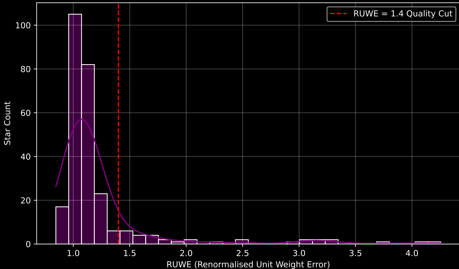
GALAH DR4 Field [1336] RUWE Distribution (n= 265)
