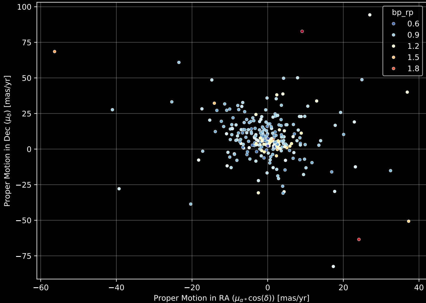
GALAH DR4 Field: [1336] Proper Motion Diagram (n= 272)
