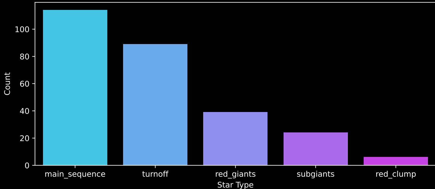
GALAH DR4 Field: [1336] Count plot of Star Type
