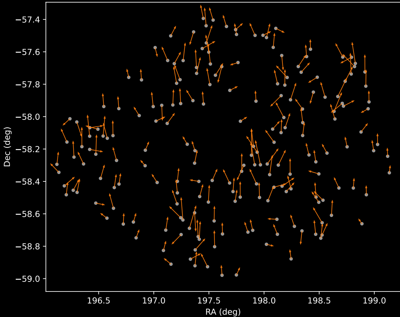
GALAH DR4 Cluster 2 Proper Motion Vectors (n=195)
